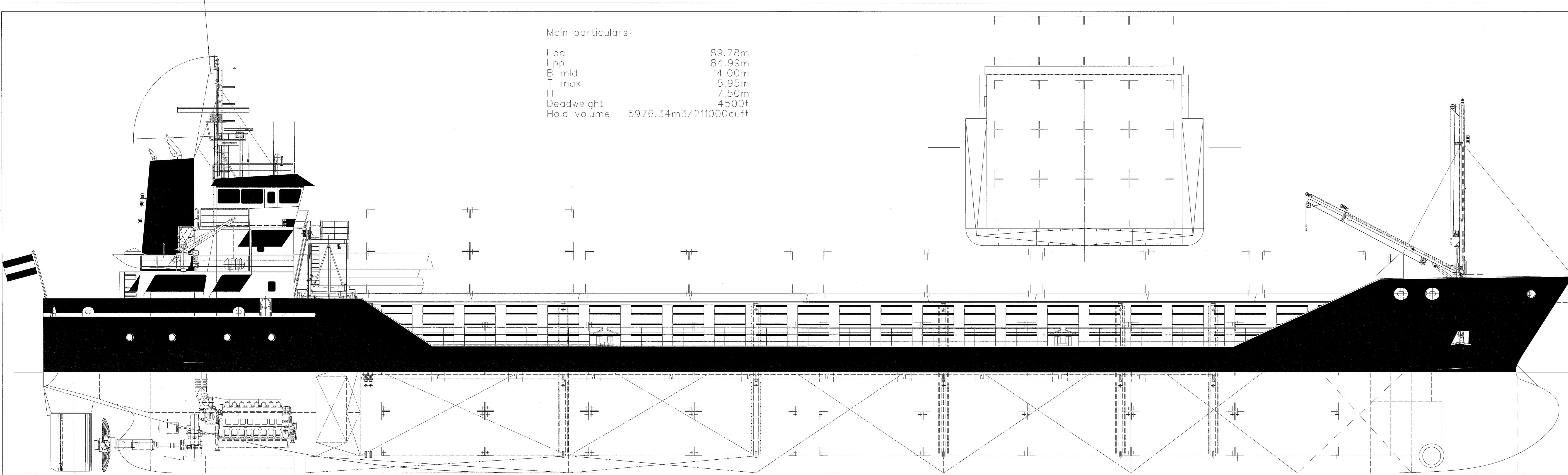
Raised Quarterdeck
